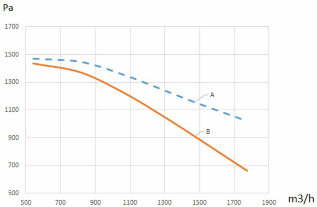
A = Fan total pressure B = Fan static pressure
